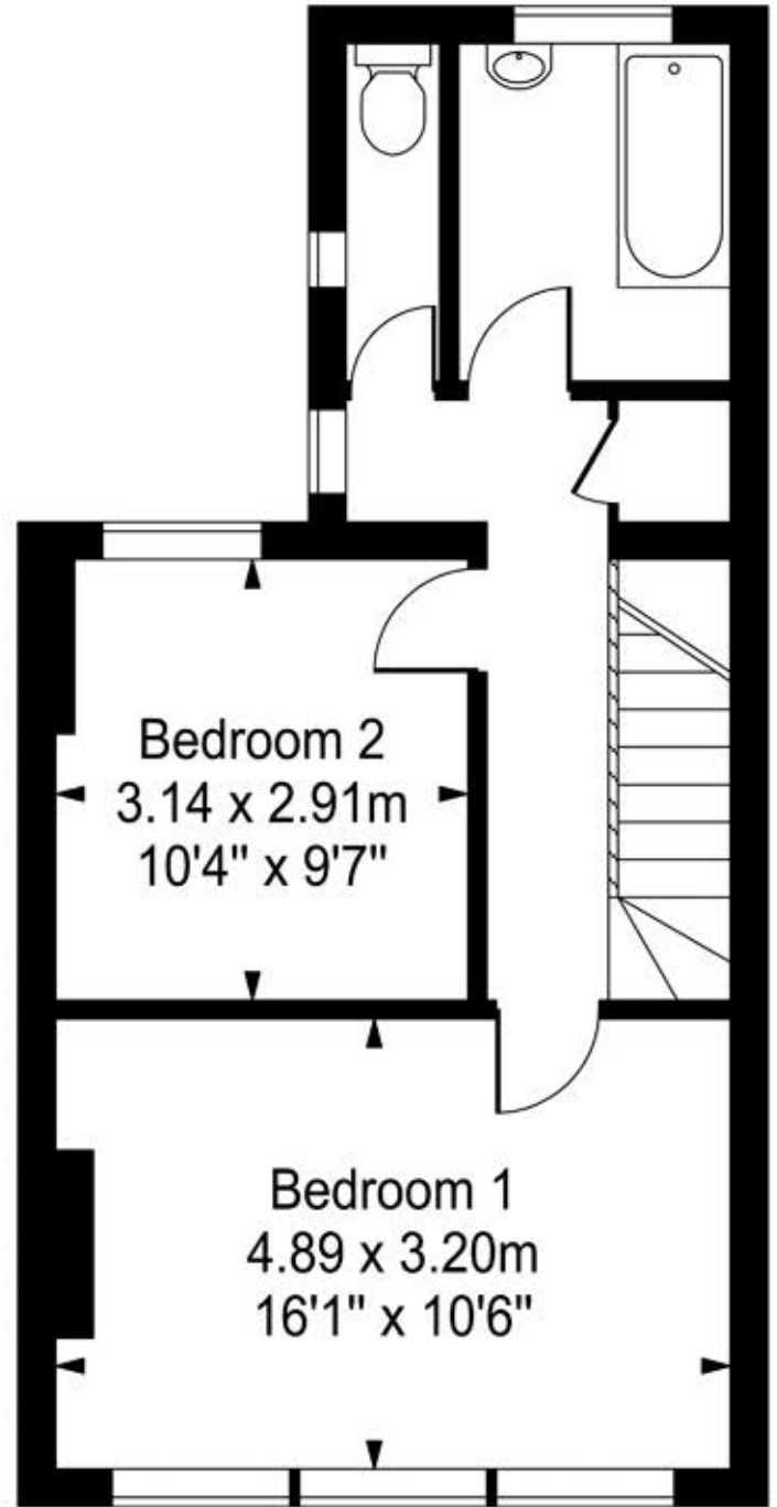
Second Floor
