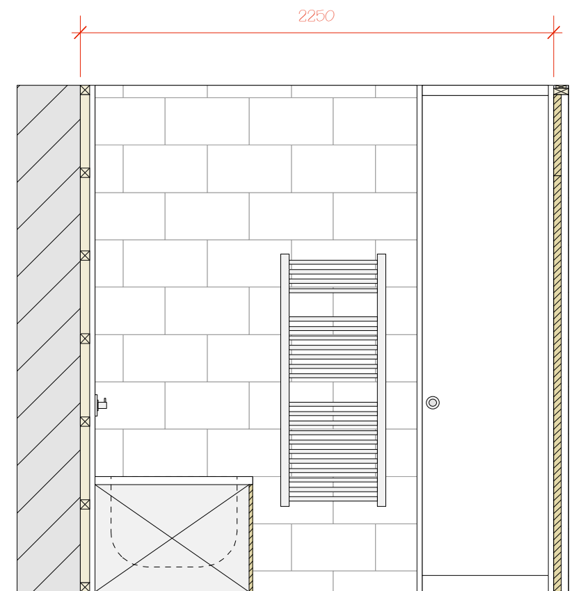
SECTIONAL ELEVATION H H
