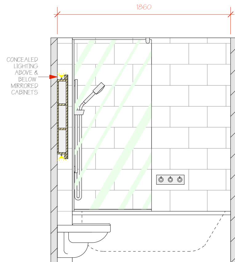
SECTIONAL ELEVATION G G
