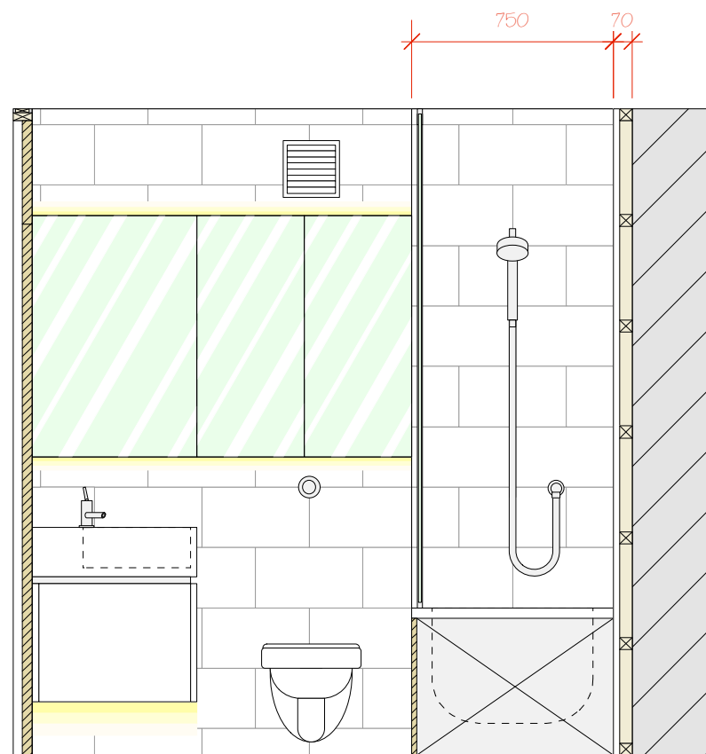
SECTIONAL ELEVATION F F
