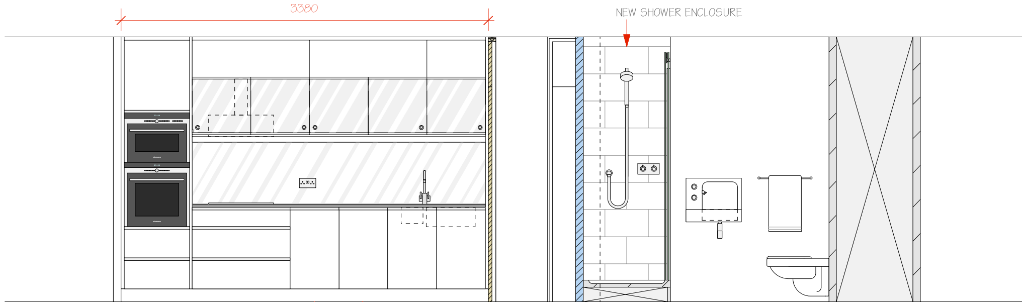
SECTIONAL ELEVATION A A
