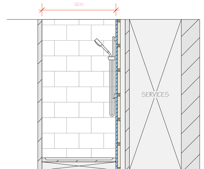
SECTIONAL ELEVATION E E (PROPOSED NEW SHOWER INTERIOR)
