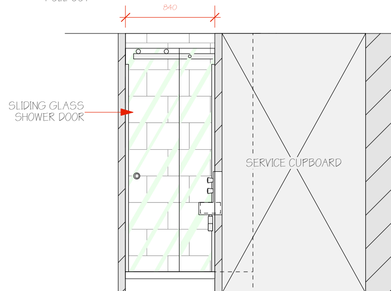
SECTIONAL ELEVATION D D (PROPOSED NEW SHOWER EXTERIOR)
