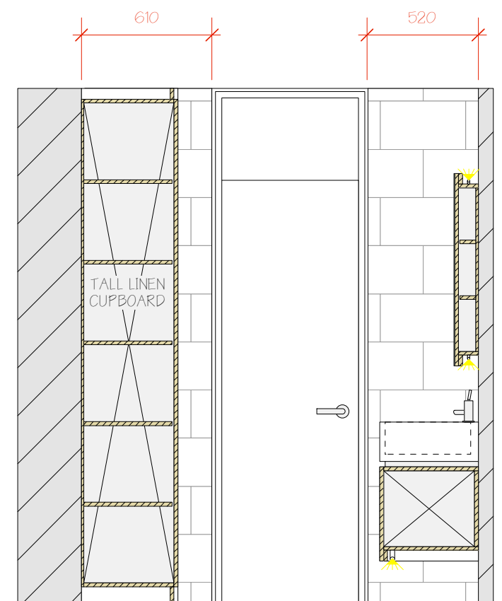
SECTIONAL ELEVATION I I
