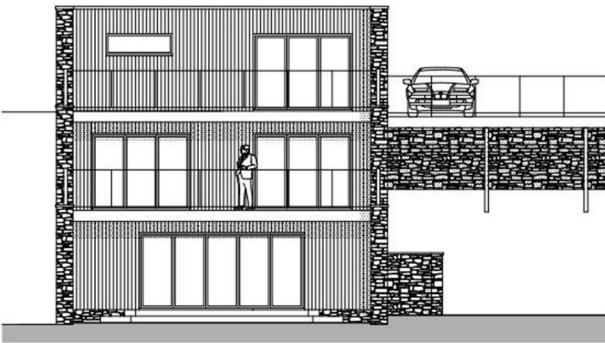
Rear NW Elevation - Plot 1
