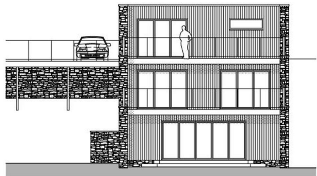
Rear NW Elevation - Plot 2
