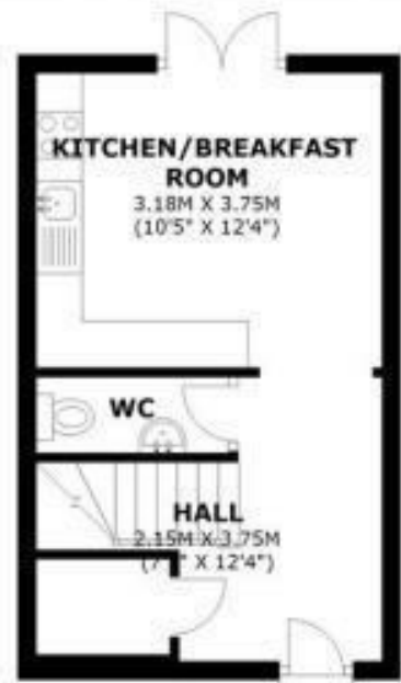
GROUND FLOOR APPROX. 23.8 SQ. METRES (255.8 SQ. FEET)
