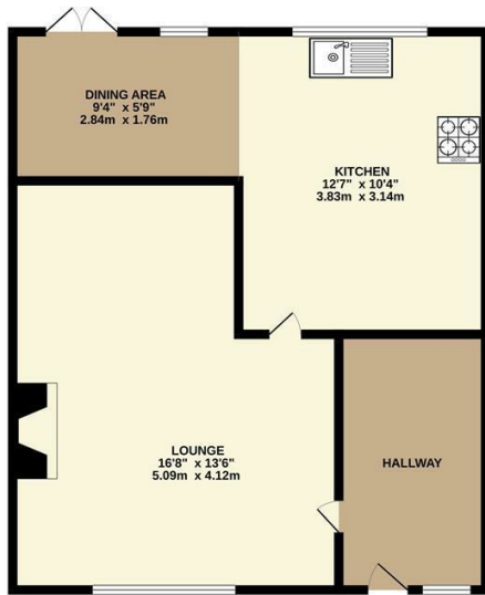
GROUND FLOOR 447 sq.ft. (41.6 sq.m.) approx.
