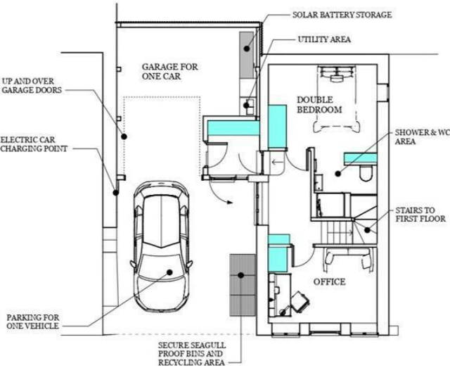
8 PROPOSED GROUND FLOOR PLAN B4 1:1000
